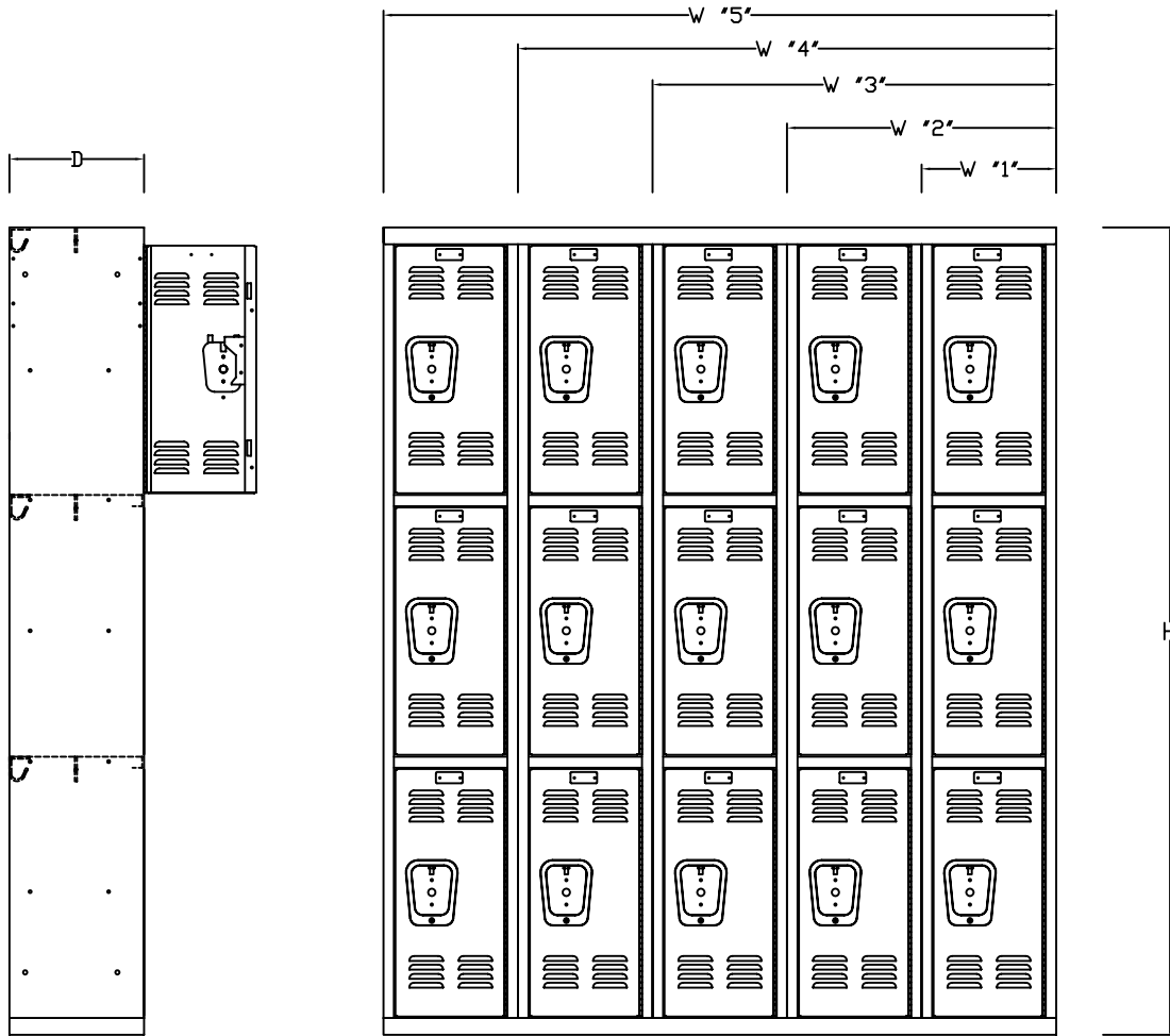
FRONT VIEW
