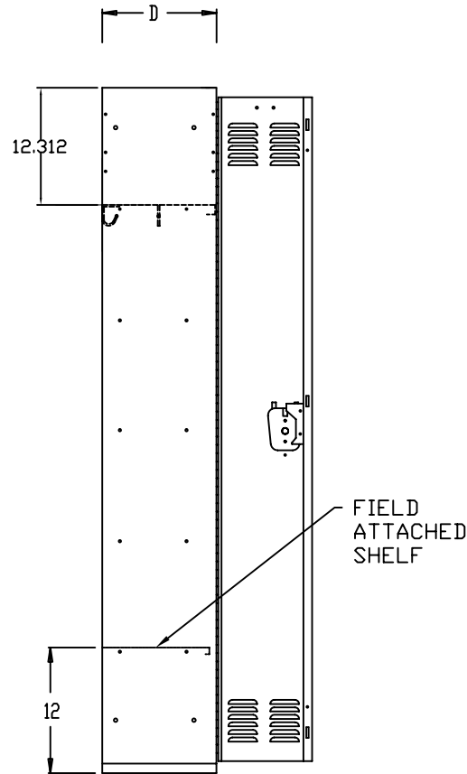
SIDE VIEW
