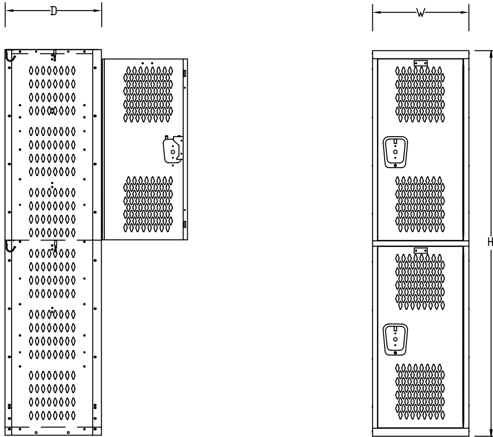
SIDE VIEW
