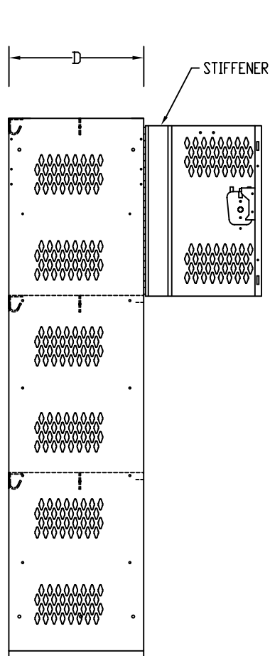
SIDE VIEW
