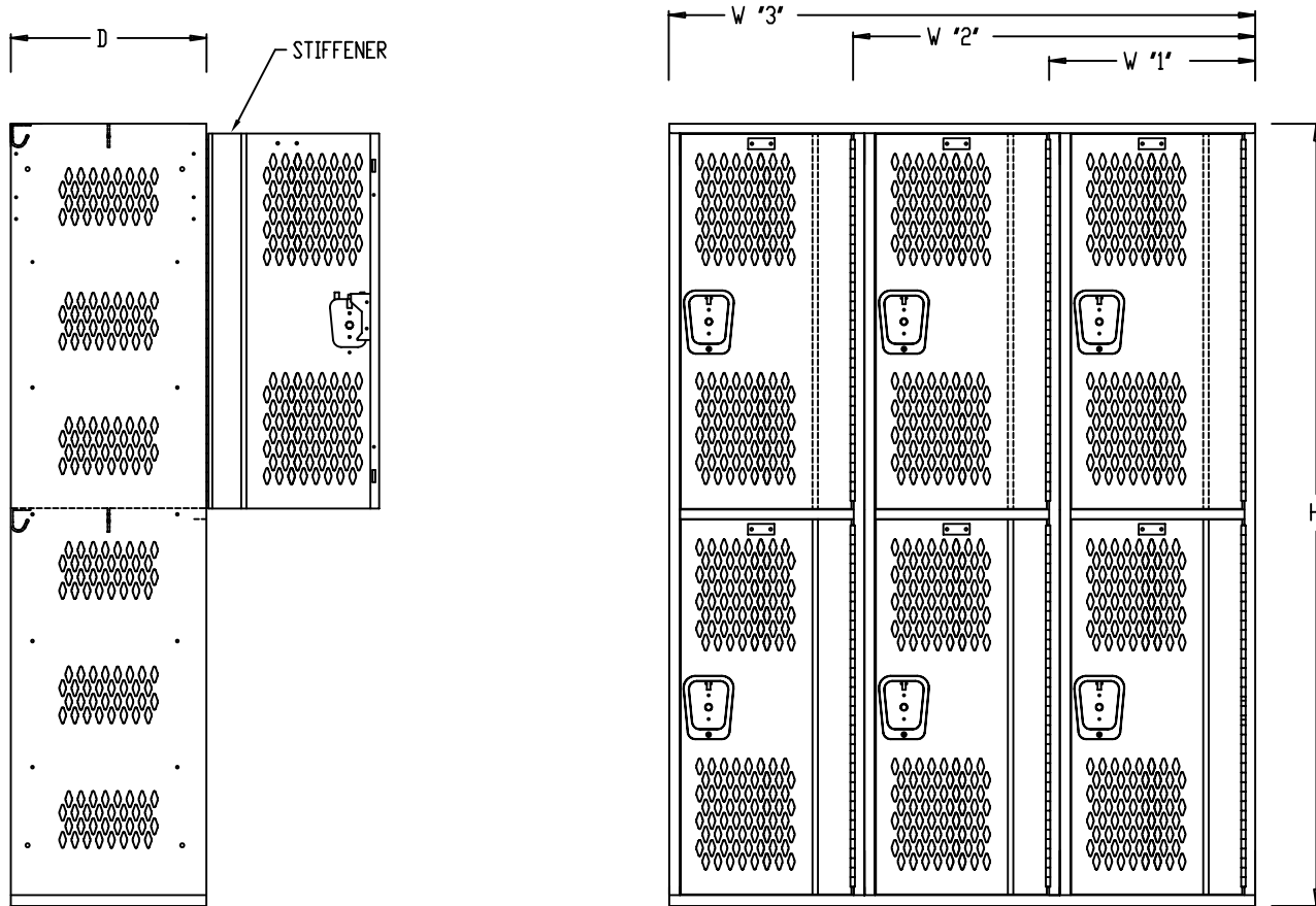
SIDE VIEW
