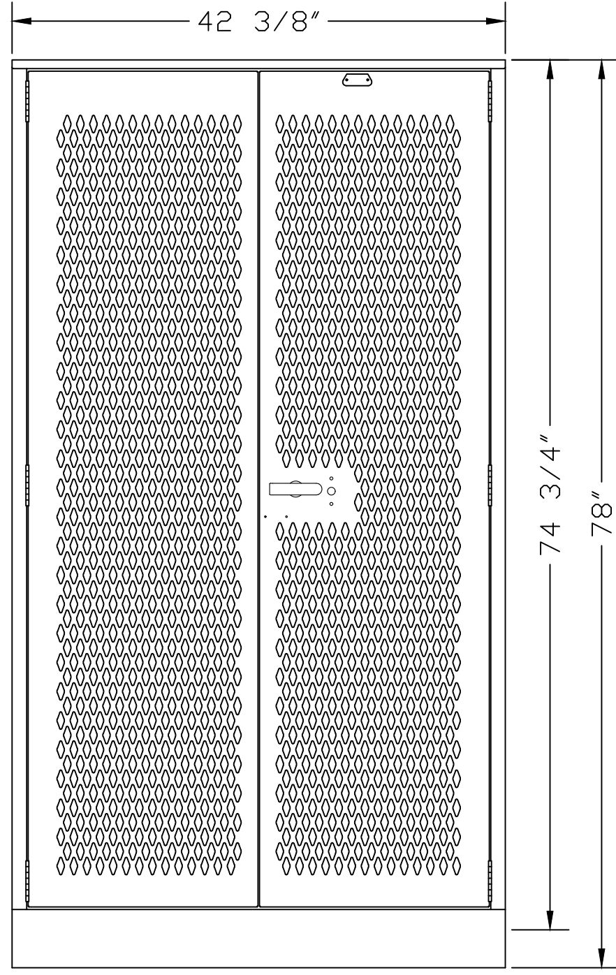
FRONT VIEW
