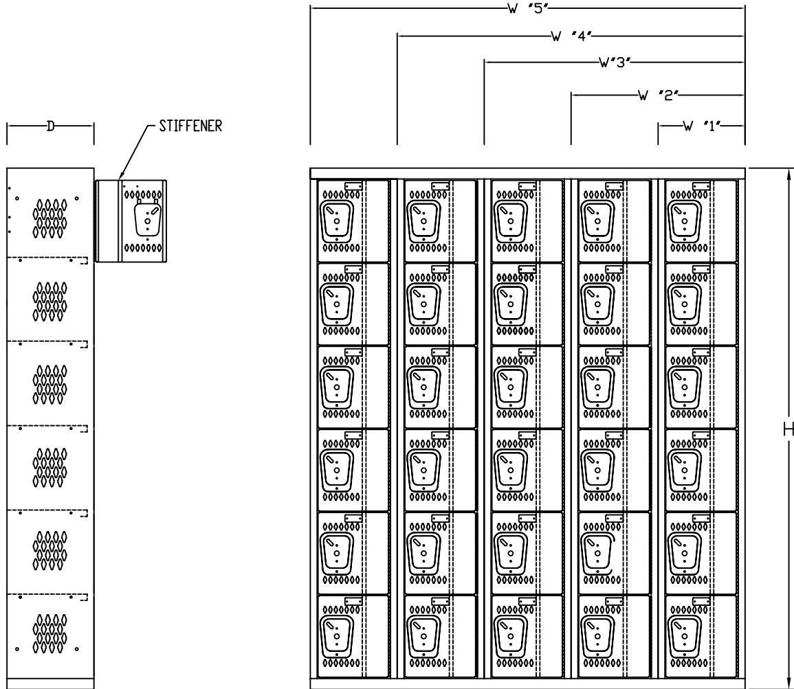
SIDE VIEW
