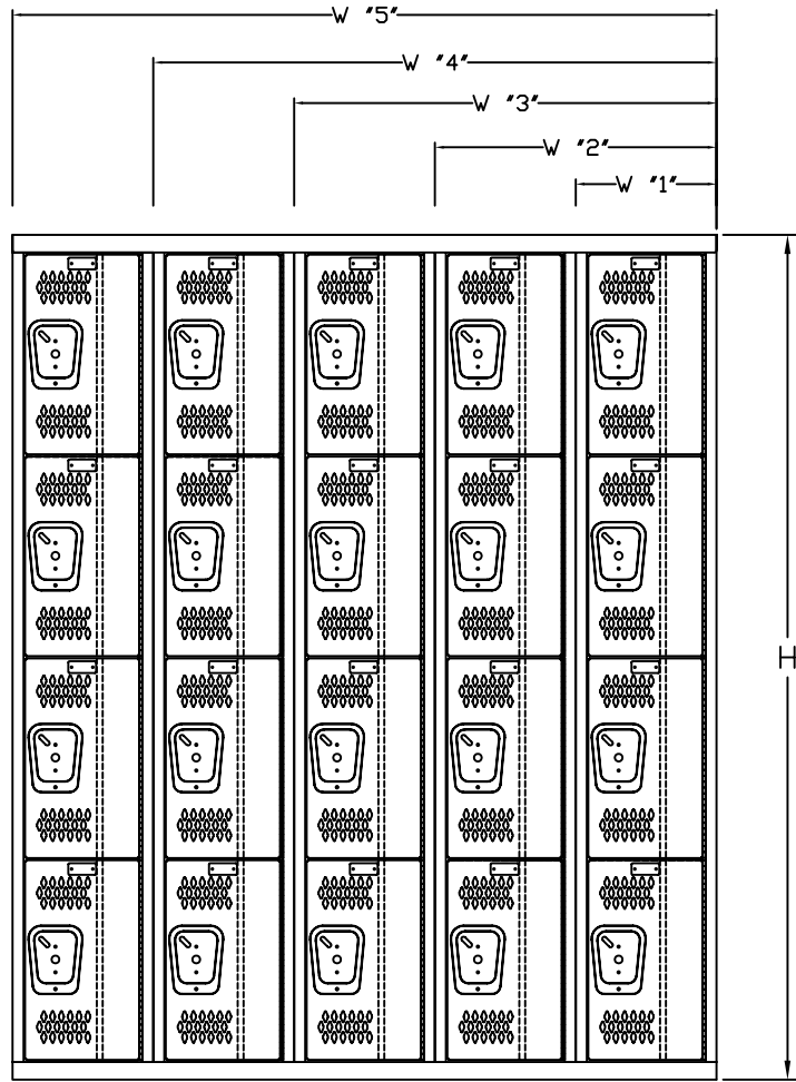
FRONT VIEW
