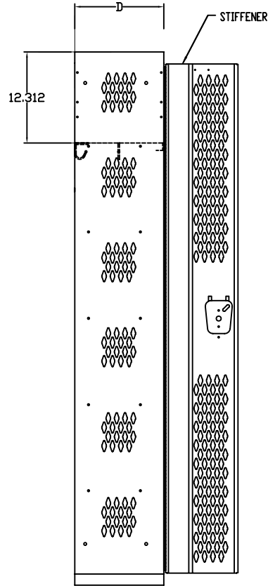
SIDE VIEW
